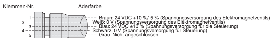
Anschlüsse
